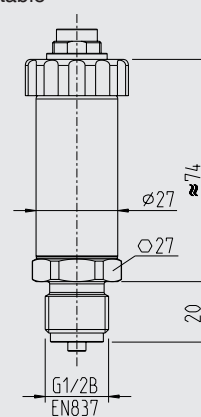
Conector circular M16 x 0,75 IEC 61076-2-106 (5 pins) ajustable
