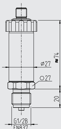
Conector circular M12 x 1 IEC 61076-2-101 A-COD (4 pins) ajustable
