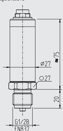
Conector circular M16 x 0,75 IEC 61076-2-106 (5 pins) no ajustable
