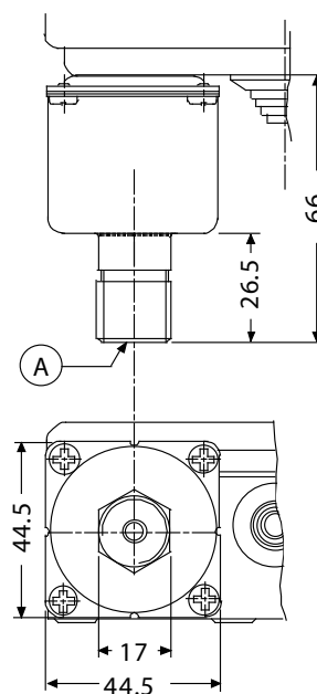
Figure 8: Ranges 0 to 1 bar and 0.2 to 4 bar A. G 3/8
