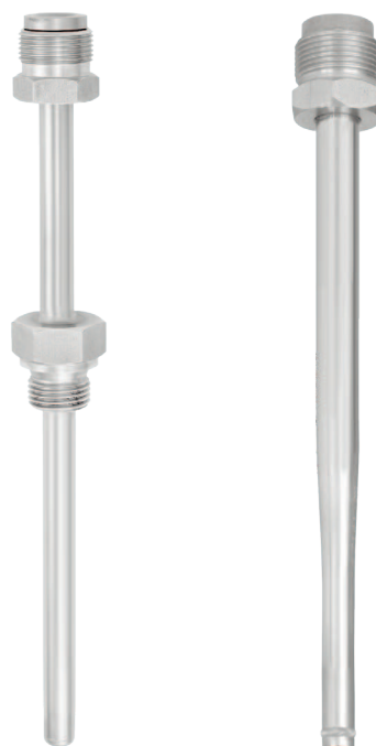
Fig. left: Threaded thermowell, model TW35-4 (Form 2G) Fig. right: Push-in/weld-in thermowell, model TW35-3 (Form 3)
