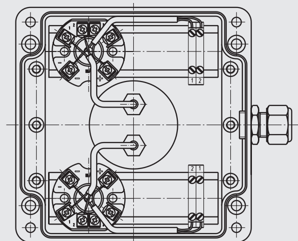
Transmisor a borne
