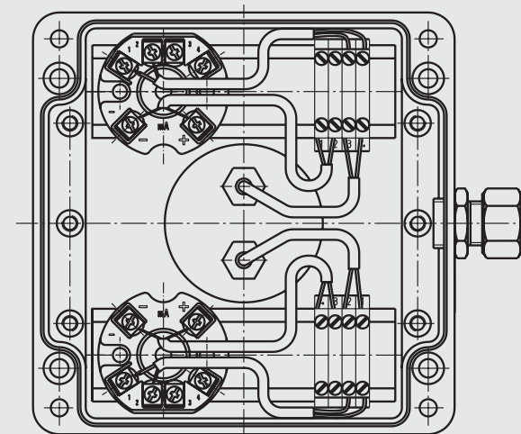
Borne a transmisor a borne
